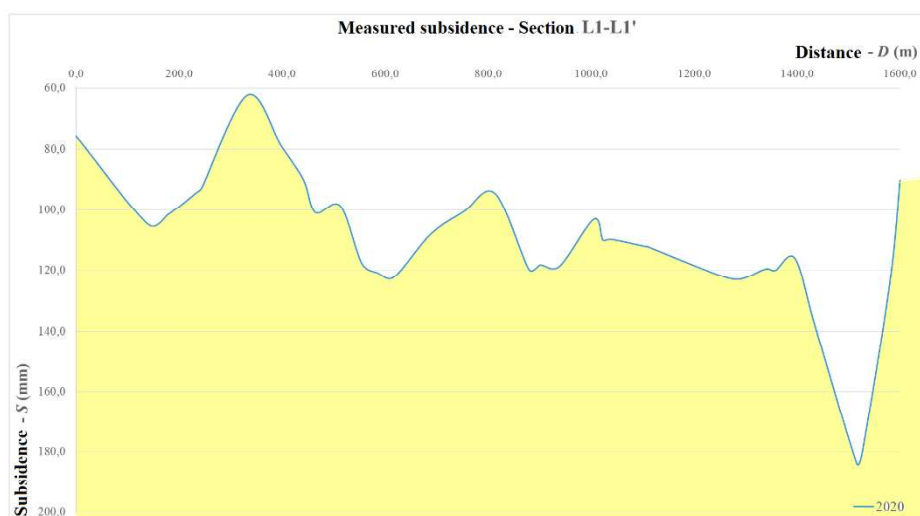
Figure 4. Subsidence measured in 2020 - E-W longitudinal section
