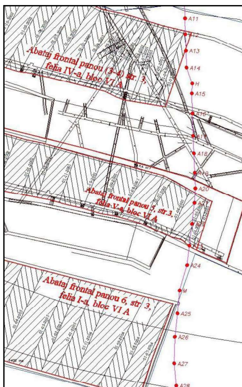
Figure 14. Situation plan for the exploitation of seam 3, block VI A, panels 3-4, 5, and 6 at the Livezeni mine
