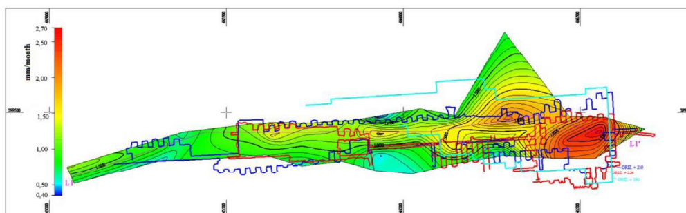
Figure 10. Predicted subsidence speed for 2030 (after mining of horizon +190 m) - scalar representation in the plan
