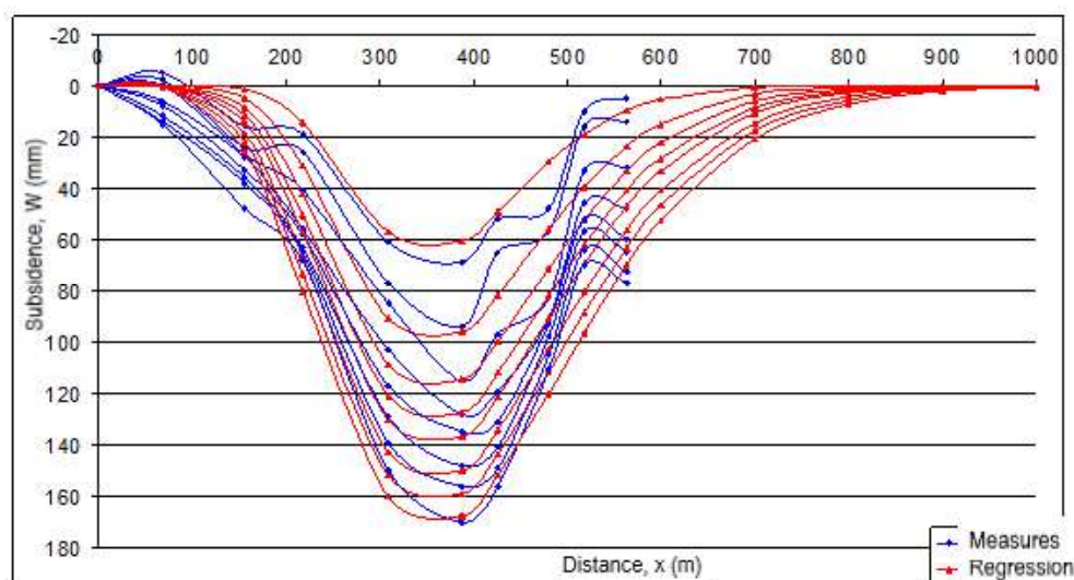
Figure 30. Tracking the displacement and deformation of the land surface following the exploitation of seam 3, block V, panel 1, at the Uricani mine [9]
