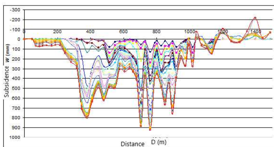
Figure 15. The diving curves followed in time at Livezeni mine [9]
