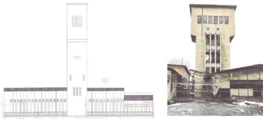
Figure 6. Center Shaft head frame [9]
