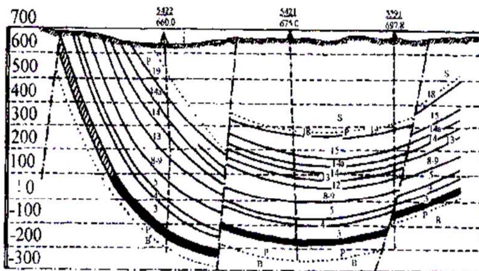
Figure 5. Structure of coal seams in the Jiu Valley mining basin
