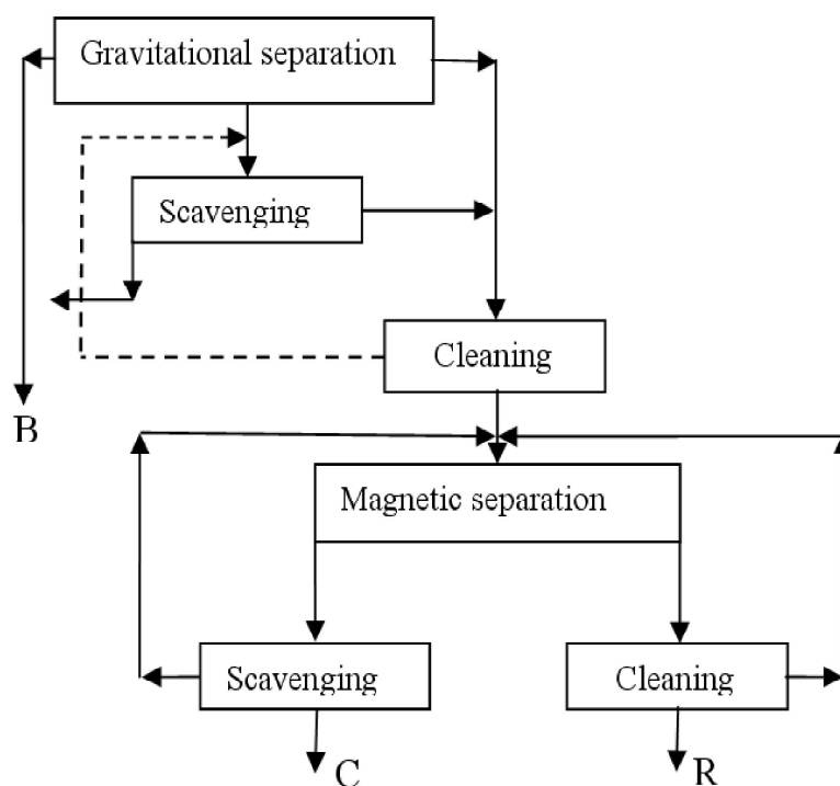
Figure 1. The processing of ash scheme [2]
