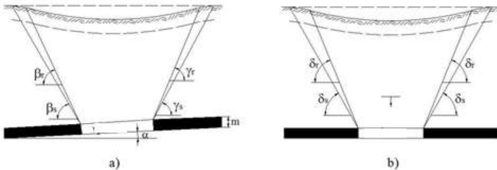
Figure 1. Representation of subsidence and breaking angles [12]: a) on inclination; b) on the direction
