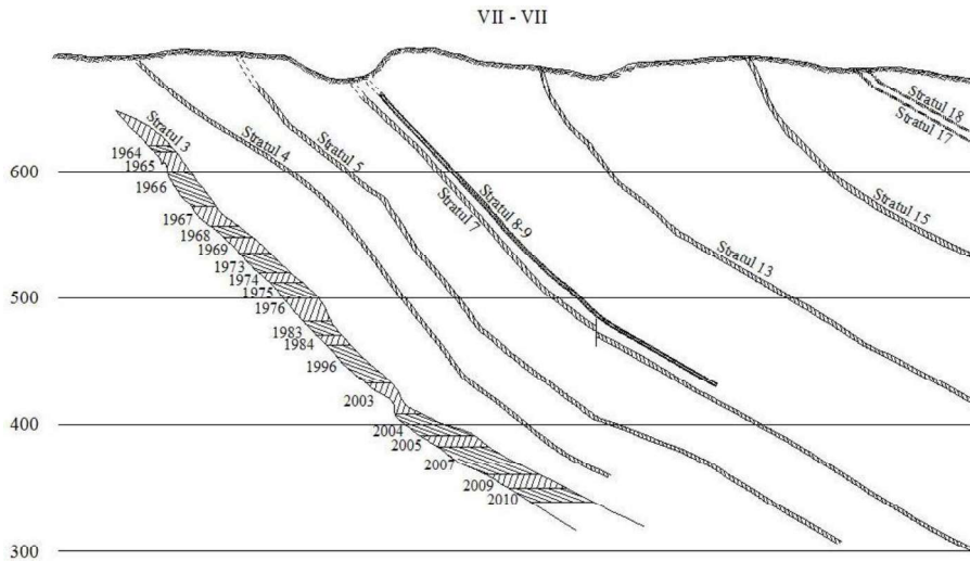
Figure 19. Vertical cross section, Vulcan mine [9]
