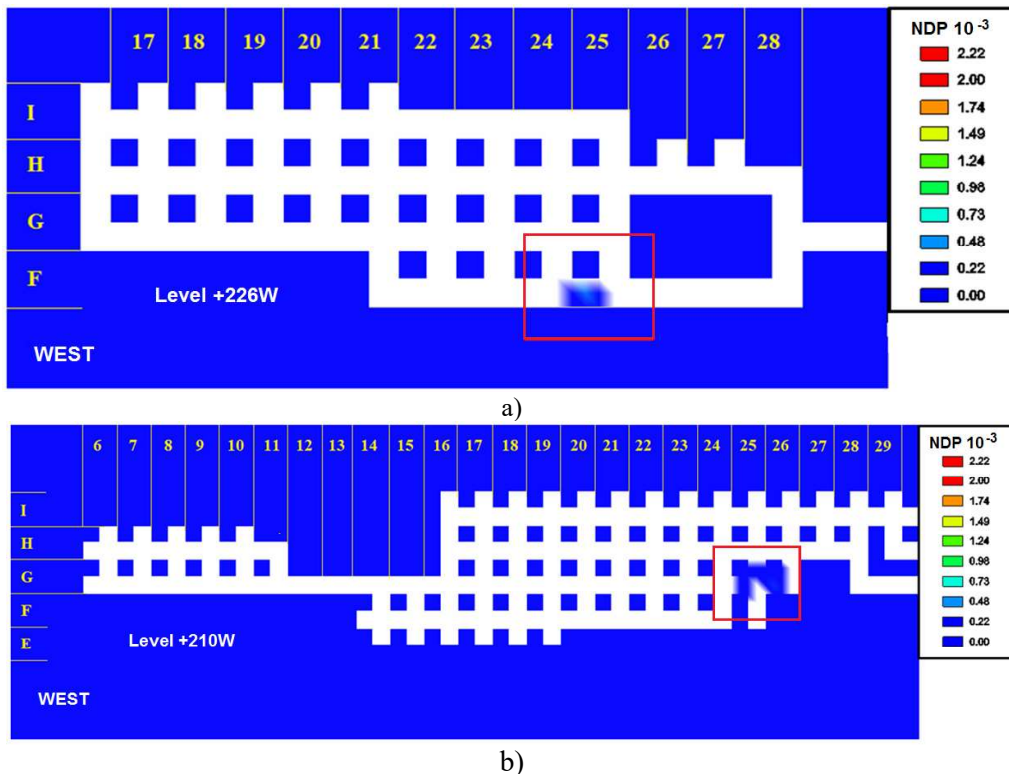
Figure 3. Situation plan of the horizons in the western side of the Ocele Mari Salt Mine: a) +226m; b) +210m; (with the distribution areas of the NDP plastic deformation norm)
