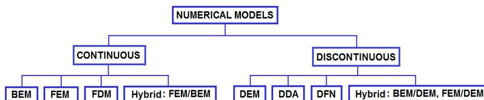
Figure 1. Classification of numerical models used in the analysis of rocks stability and mining excavations
