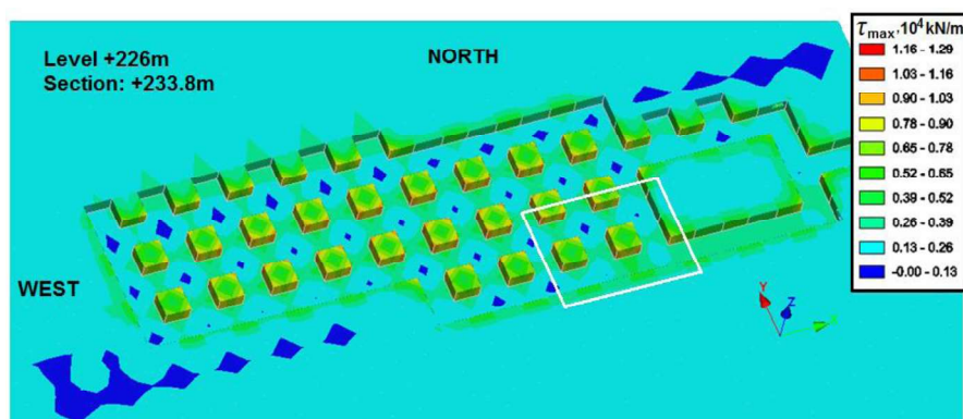
Figure 6. Horizontal view of maximum shear stresses, in \text{kN/m}^2 a) Level +226 m-east; b) Level +226 m-west
