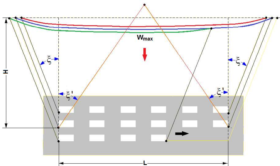
Figure 1. Development of the subsidence trough following the successive exploitation of the levels
